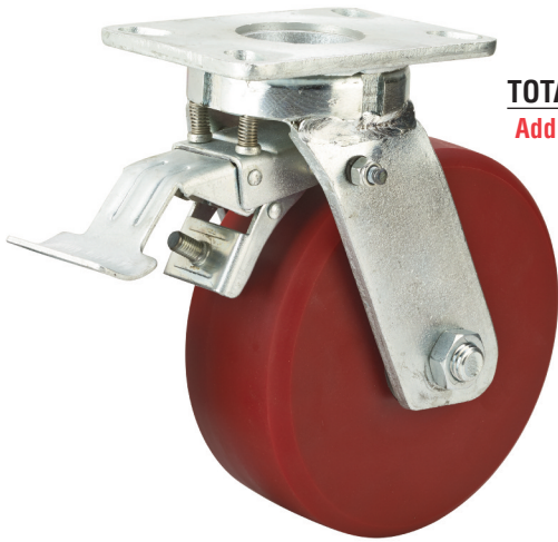
NEW TRAILING SIDE TOTAL LOCK SWIVEL CASTER No need to move cots back and forth for finding the brake pedal. Add TLT to swivel caster number Available in 6" & 8"
