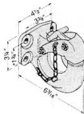
PH10 PINTLE HOOK
