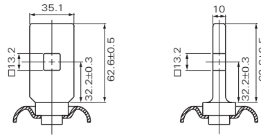
K1 Flange Fitting
